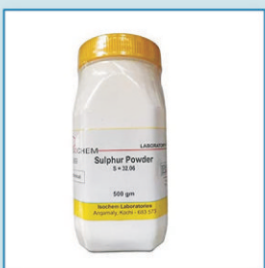
SULPHUR POWDER
