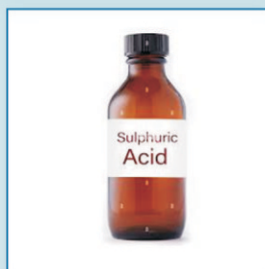
SULPHURIC ACID
