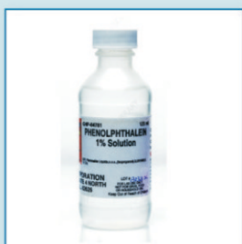
PHENOPHTHALENE
