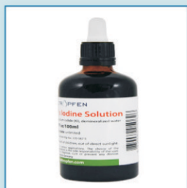
FODLINE SOLUTION
