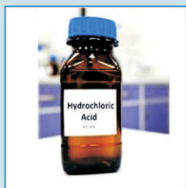
HYDROCHLORIC ACID
