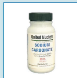
SODIUM CARBONATE
