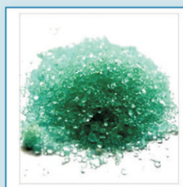
FERROUS SULPHATE
